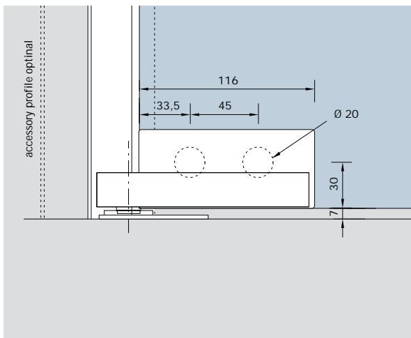
view DORMA EA with floor pivot bearing
