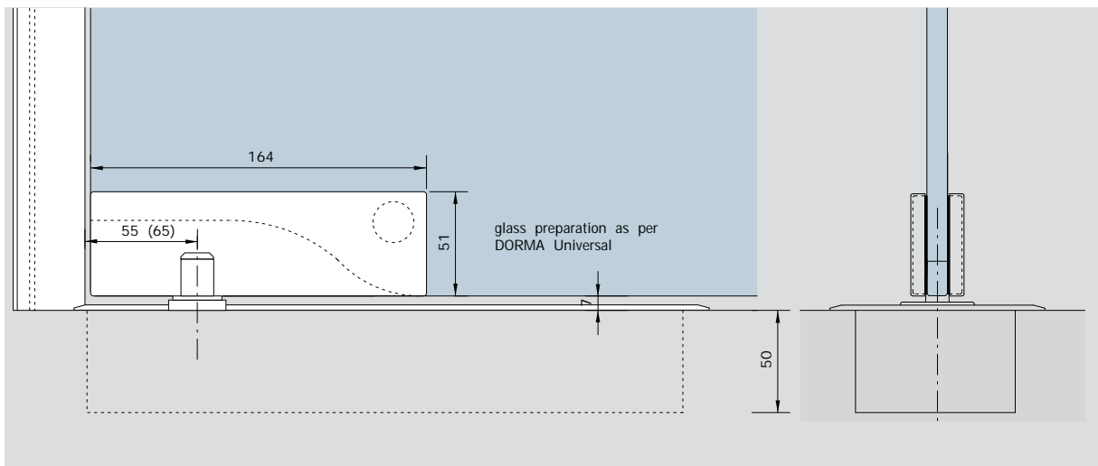
view DORMA Universal patch fitting, floor closer
