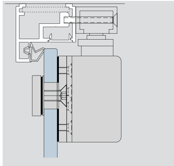
slide channel closer DORMA TS 92 on frame profile
