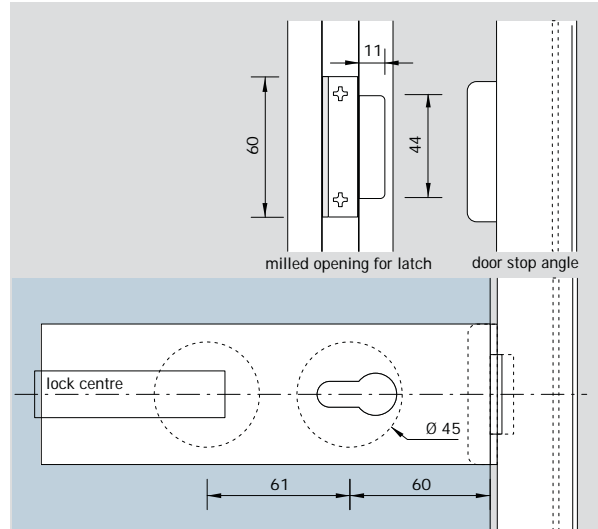
view DORMA lock Studio Classic
