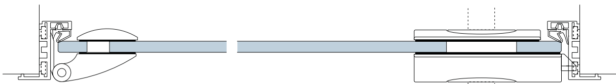
Deubl AT 23 E with DORMA special hinge ARCOS Art. no. 25.450, lock ARCOS Office
