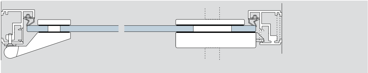
Deubl AT 44 - with DORMA Junior (Office, Office Classic)
