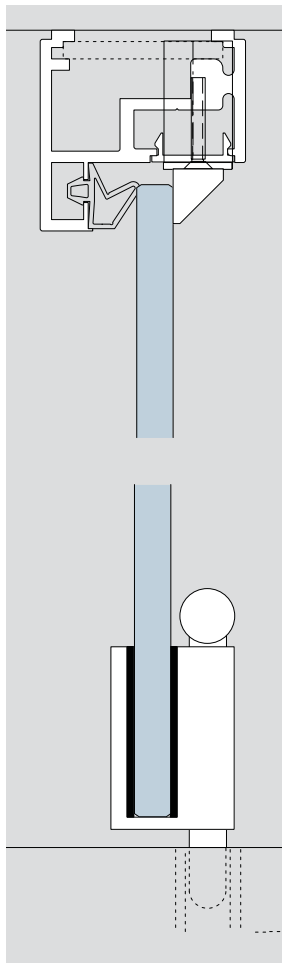
frame profile
