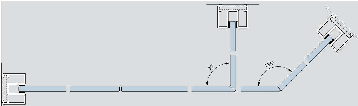
Deubl PT 35 fixed glazing
