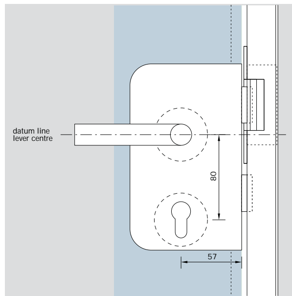
view lock Junior Office
