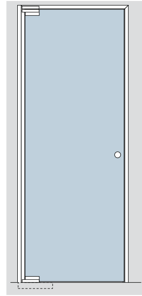
Type C Deubl AT 44 EA 3 sided frame profile with 1 sided accessory profile for floor closer (BTS).
