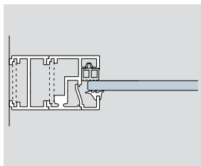
Deubl AT 44 fixed glazing with accessory profile
