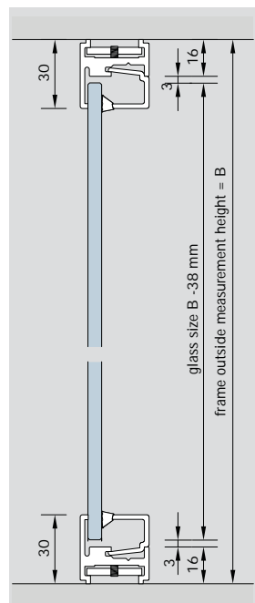
sectional cut door frame surround
