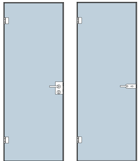
Deubl AT 23 Single acting door frame
