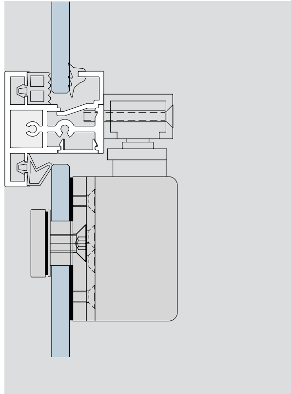
slide channel closer DORMA TS 92 on rung profile
