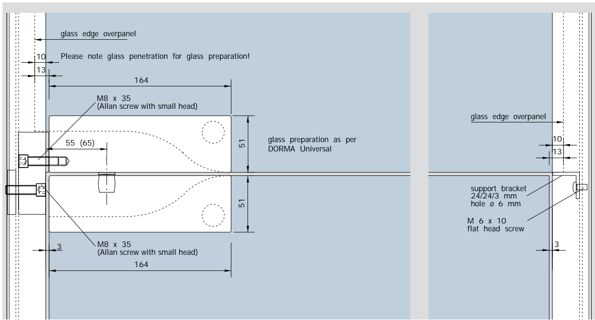
view DORMA Universal patch fitting
