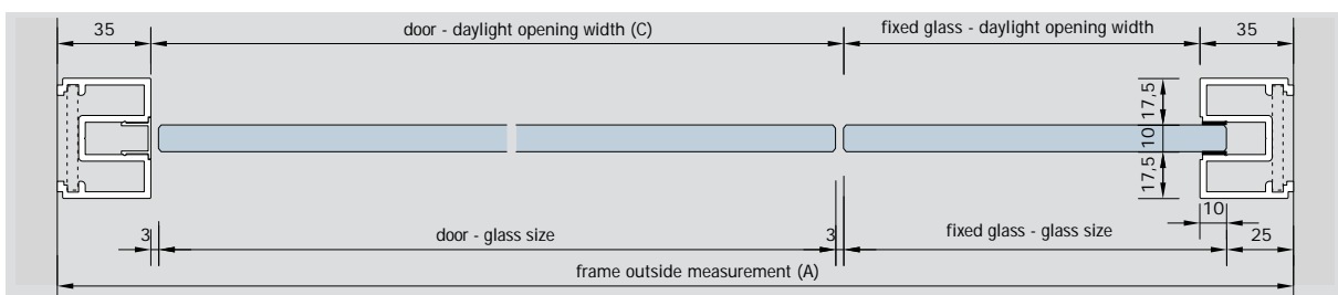
plan / door with fixed glazing
