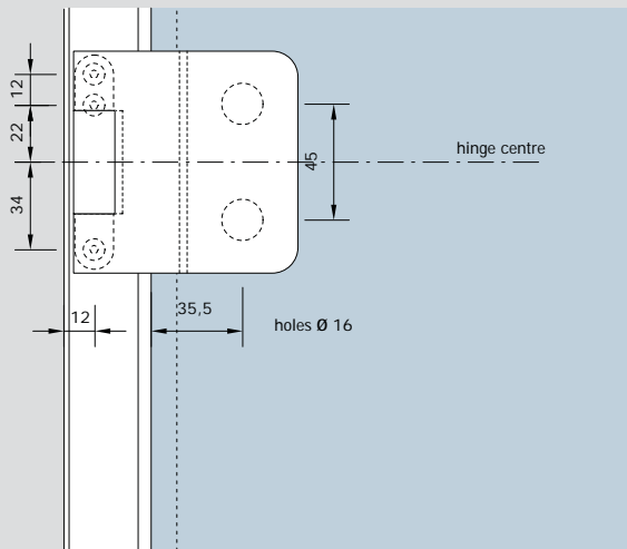
Standard hinge Studio Rondo Studio Rondo with screw-on frame pivot
