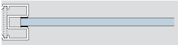
Deubl PT 35 frame profile with glass penetration
