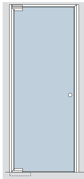
Type B Deubl AT 44 EA 3 sided frame profile with 2 sided accessory profile for floor closer (BTS).
