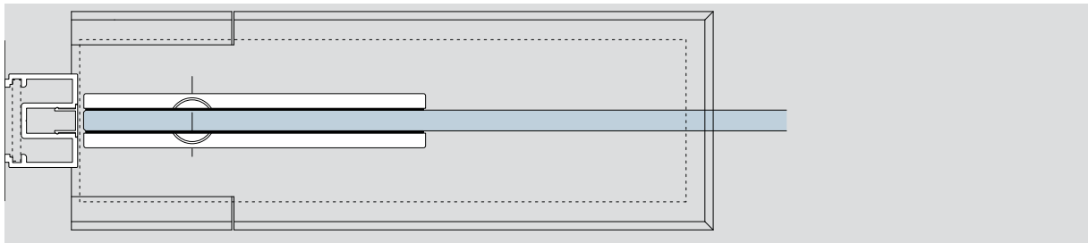
Deubl PT 35 with DORMA Universal patch fitting, floor closer BTS 75 V
