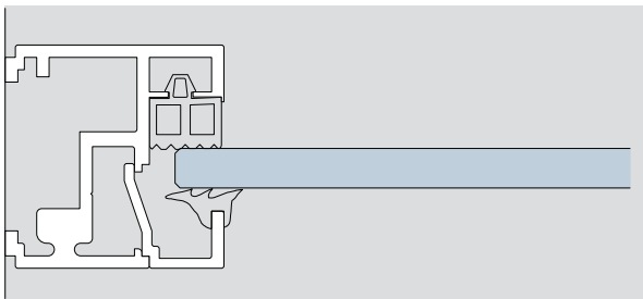
Deubl AT 44 - fixed glass
