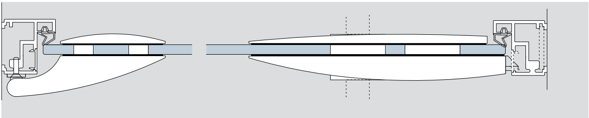
Deubl AT 44 - with DORMA ARCOS Studio
