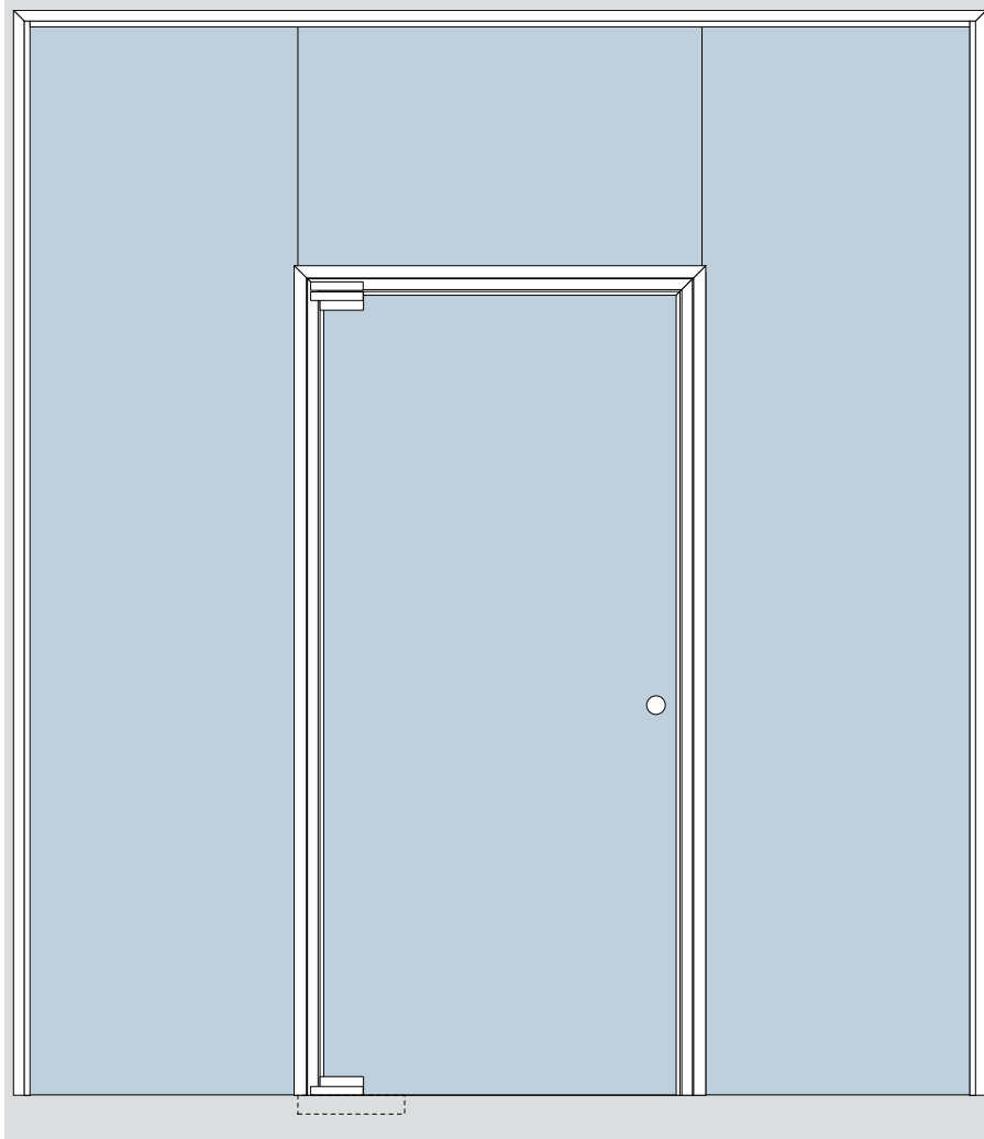
Delicate construction for fixed side lites with overpanel and centre positioned single acting door - The combination of frames Deubl AT 44 and Deubl PT 35.
