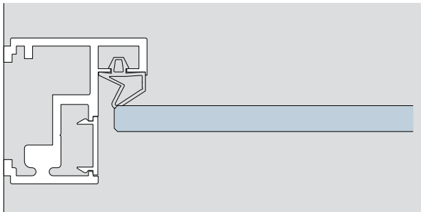
Deubl AT 44 - frame profile
