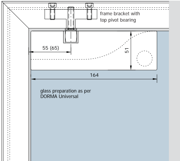
view DORMA Universal top patch fitting
