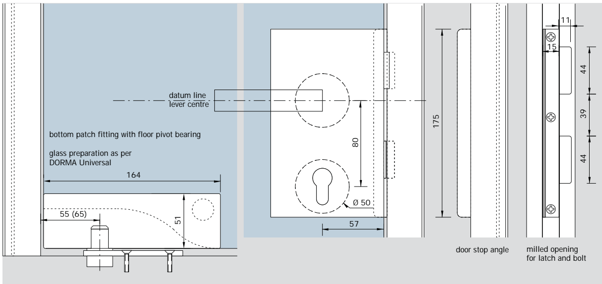
view DORMA Universal bottom patch fitting
