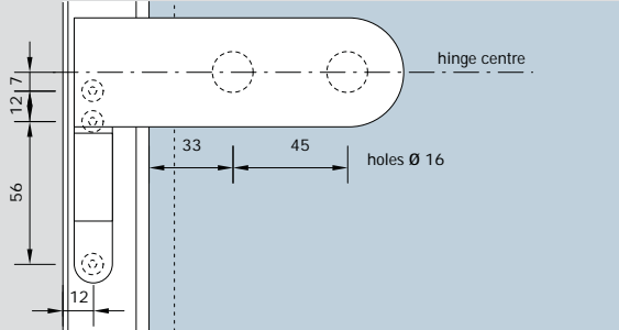
overpanel fixing adjustable angle bracket
