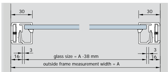
plan door frame surround
