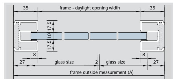
plan / fixed glazing with two elements
