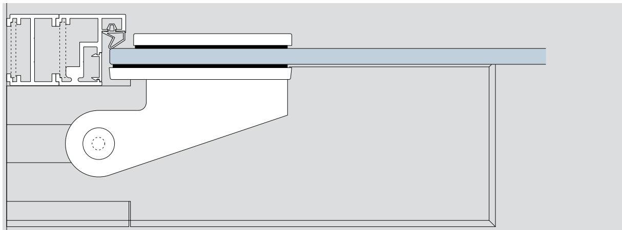
Deubl AT 44 with DORMA EA, and floor closer DORMA BTS 75V
