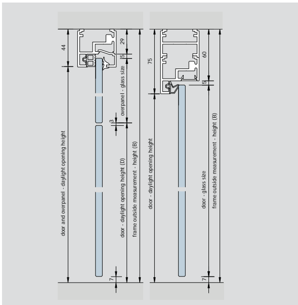
sectional cut
