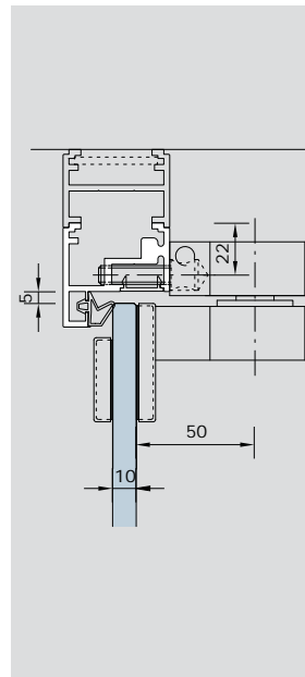
sectional cut DORMA EA top patch fitting
