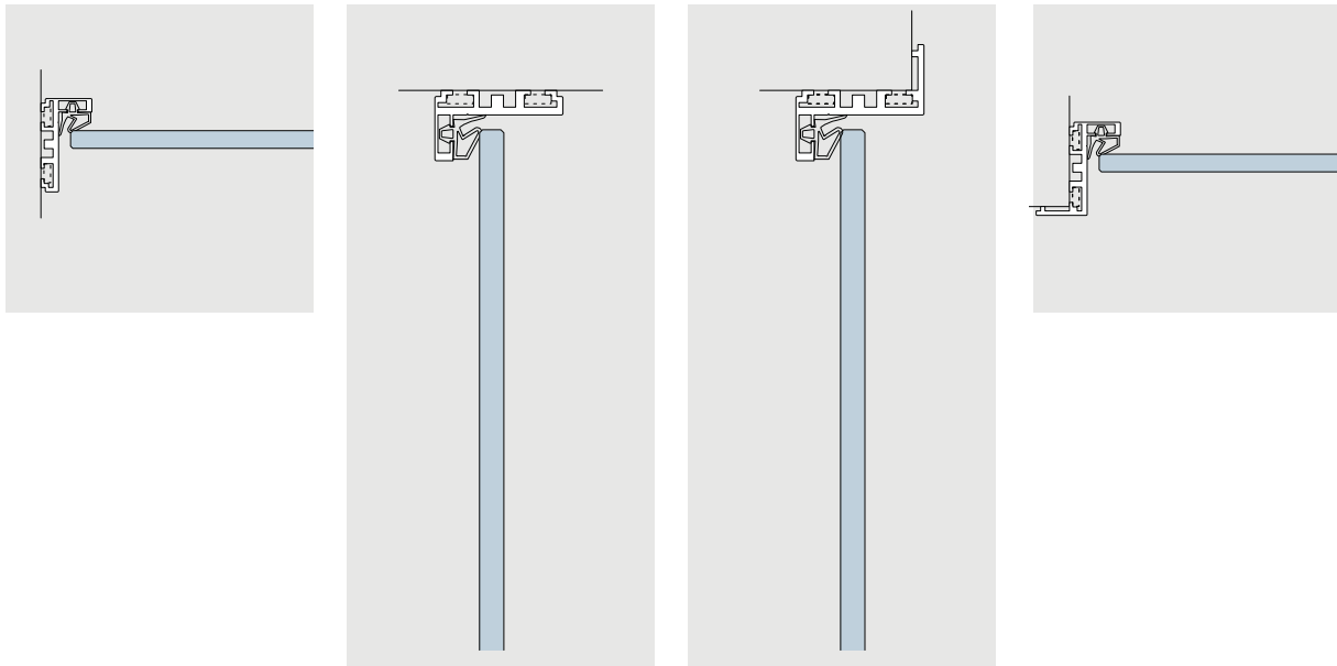
Single acting door frame AT 23
