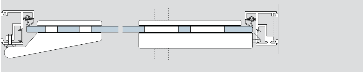
Deubl AT 44 - with DORMA Studio (Classic, Rondo)
