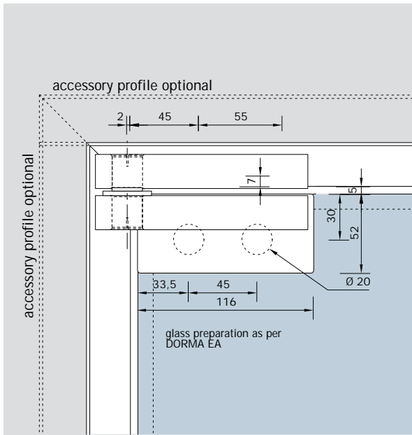
view DORMA EA top patch fitting
