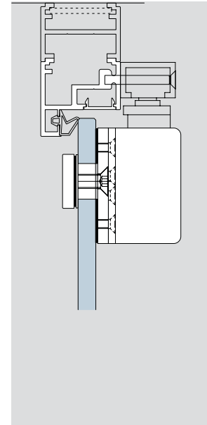
Slide channel door closer DORMA TS 92
