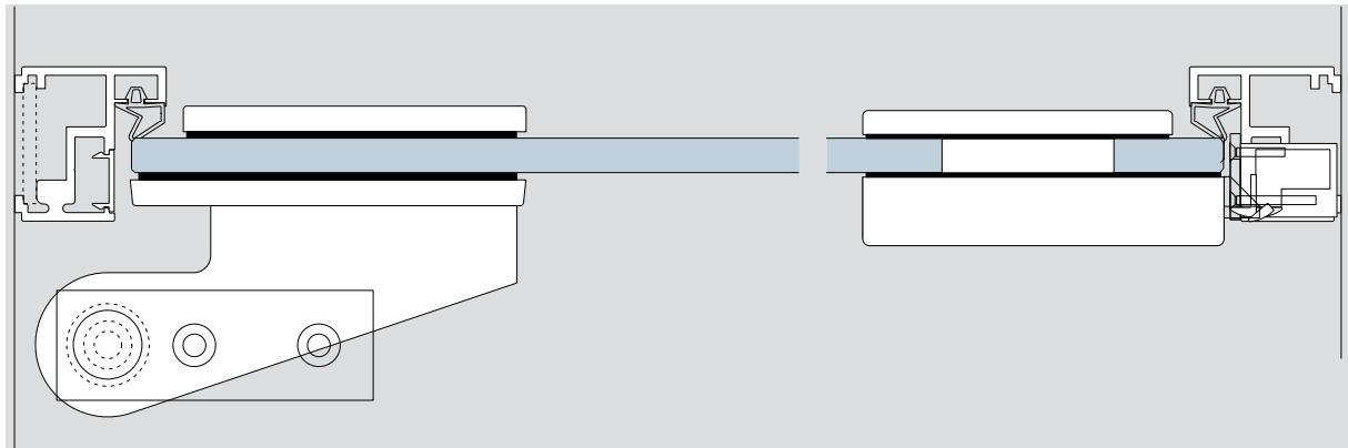
Deubl AT 44 with DORMA EA, and floor pivot bearing Art. no. 01.106
