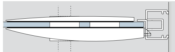
plan lock DORMA ARCOS Studio
