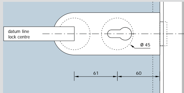
view lock Studio Rondo
