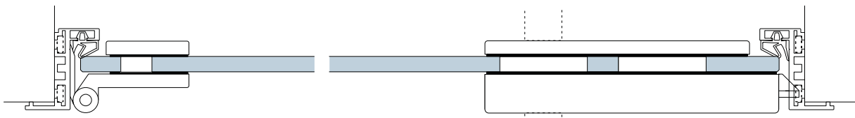
Deubl AT 23 E with DORMA special hinge Art. no. 11.294 resp. 12.050, lock Studio Rondo / Classic
