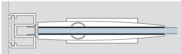
plan DORMA ARCOS Universal patch fitting
