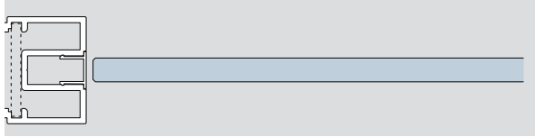
Deubl PT 35 frame profile with cover clip profile
