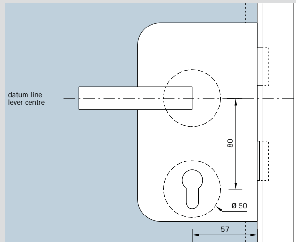
view lock Junior Office
