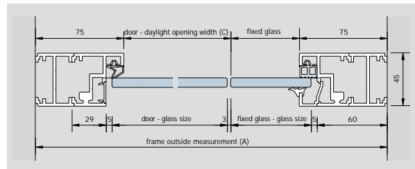
plan / door with fixed glazing Type A
