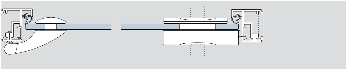
Deubl AT 44 - with ARCOS Office
