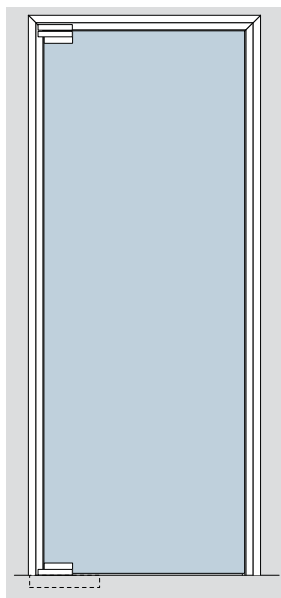
Type A Deubl AT 44 EA 3 sided frame profile with 3 sided accessory profile for floor closer (BTS).
