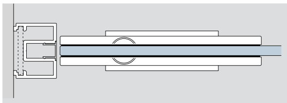
plan DORMA Universal patch fitting
